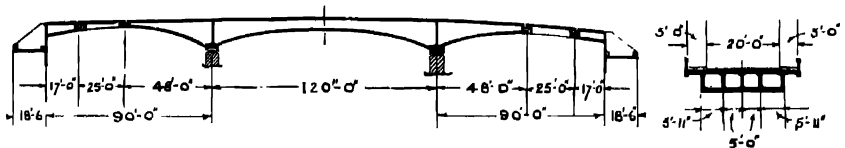
Fig. 356.—Road Bridge at Wiggshall, Norfolk.
